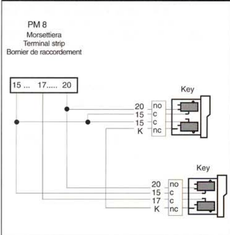
Fig. 13 - COLLEGAMENTO DI N°2 KEY - CONNECTION OF TWO KEY CONNECTION OF 2 KEY
